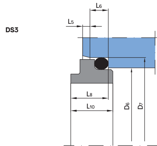
Dimension table Ø 105 – 160 mm
