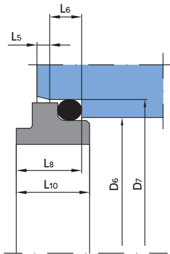
Dimension table Ø 35 – 70 mm | 1 3/8 – 2 3/4 inches
