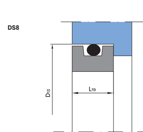
Dimension table Ø 10 – 30 mm
